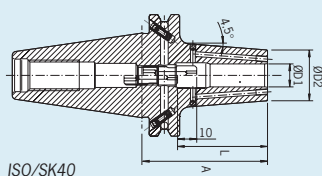
ISO/SK40
